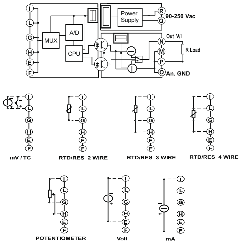
TS 4135AC: SCHEMA A BLOCCHI E COLLEGAMENTI TS-4135AC : BLOCK DIAGRAM AND WIRING DIAGRAM
