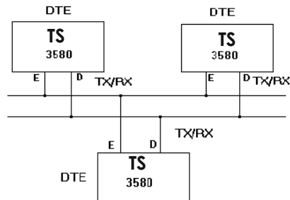
RS-485 multipoint connection
