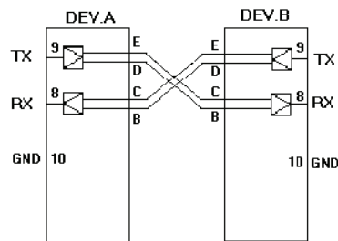
RS-422 point to point connection
