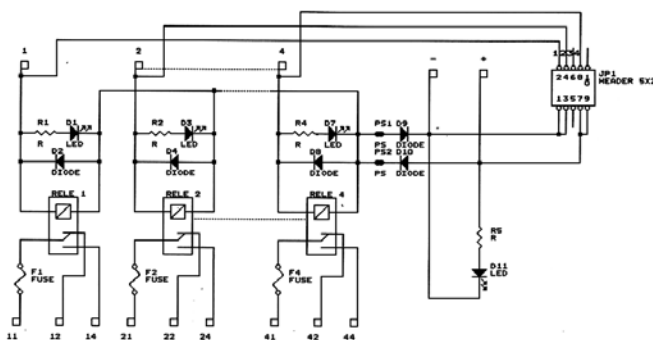
Schema a 4 relè Wiring diagram of module with 4 relays
