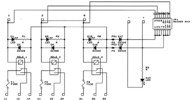
Schema a 8 relè Wiring diagram of module with 8 relays
