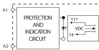
Modelli in DC DC models
