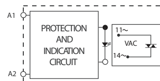
Modelli in AC AC models
