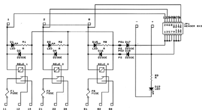
Schema a 8 relè Wiring diagram of module with 8 relays
