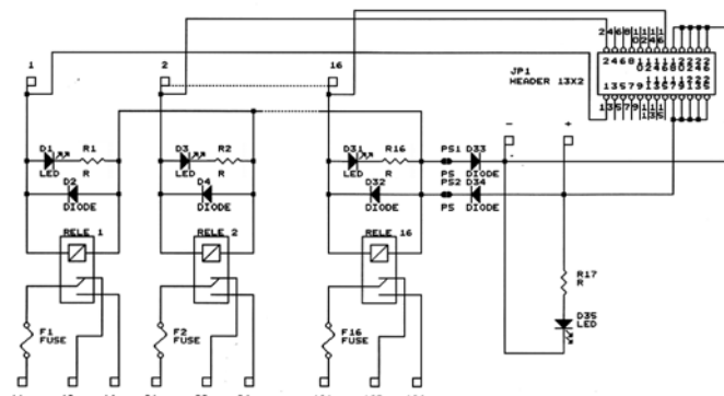
Schema a 16 relè Wiring diagram of module with 16 relays
