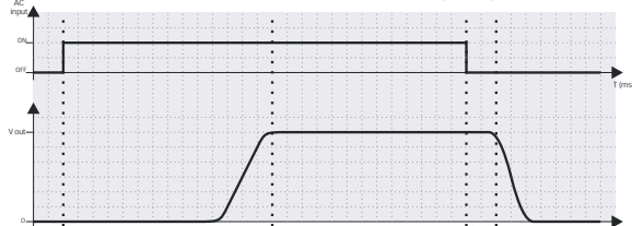
RISE TIME & HOLD-UP TIME 230VAC (Curva5)
