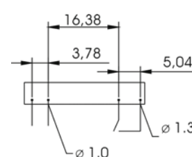
Layout fori montaggio Mounting hole Layout
