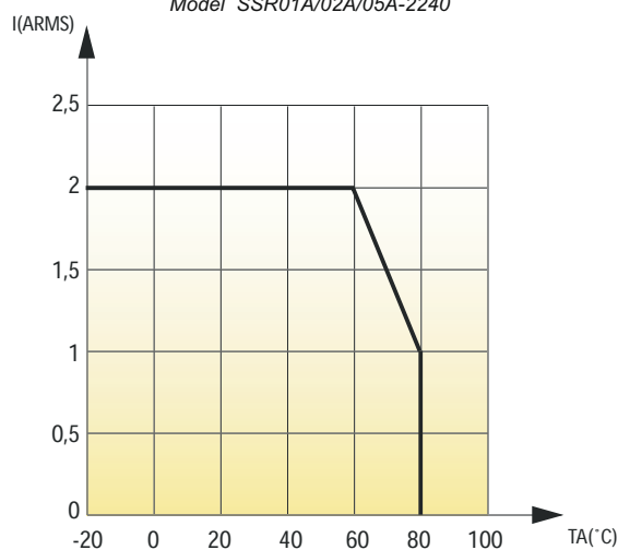
Modello SSR01A/02A/05A-2240 Model SSR01A/02A/05A-2240
